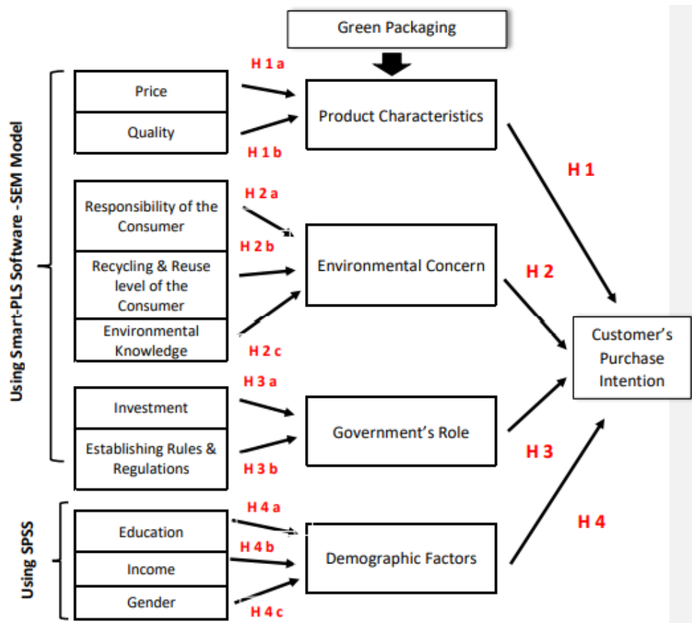
Figure 2: Hypothesis testing under the conceptual frame work
